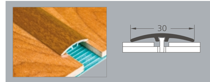
70 (035) invisible fixing, 0-8 mm level difference color : 01, 02, 03, 04, 05, 06, 017, 116, 117, 308, 309, 310, 315, 316, 350, 417, 617, 717, 88
