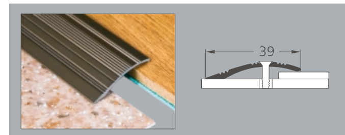
3326 visible fixing, 0-16 mm level difference color : 01, 02, 017, 116, 317, 217, 417
