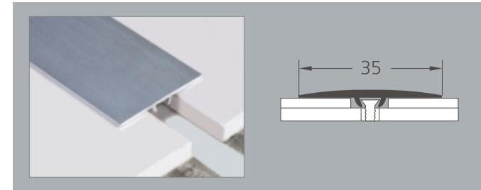
72 (033) invisible fixing, 0-13 mm level difference color : 01, 02, 03, 04, 05, 06, 017, 116, 117, 308, 309, 310, 315, 316, 350, 417, 617, 717, 88
