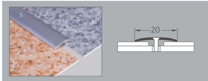
110 visible fixing, 0-3 mm level difference color : 01, 02, 03, 04, 05, 06, 017, 116, 117, 308, 309, 310, 315, 316, 350, 417, 617, 717, 88
