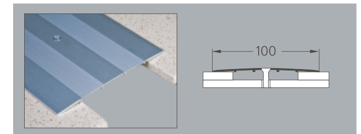
10 visible fixing, no level difference color : 01, 02
