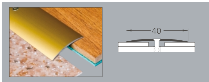
120 visible fixing, 0-5 mm level difference color : 01, 02, 04, 06, 017, 116, 117, 308, 309, 310, 315, 316, 350, 417, 617, 717
