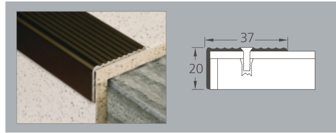
664 visible fixing color : 01, 02, 04, 06, 117, 310, 315, 417, 617
