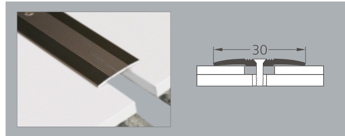
3328 visible fixing, no level difference color : 01, 02, 88
