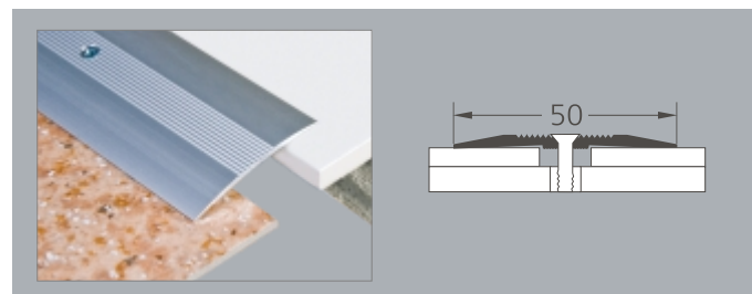
3584 visible fixing, no level difference color : 01, 02
