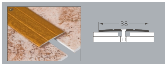
140 visible fixing, no level difference color : 01, 02, 04, 06, 117, 116, 117, 310, 315, 417, 617, 717
